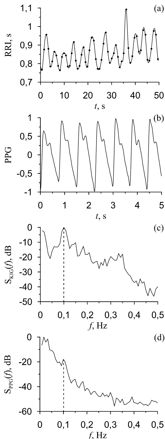
Figure 8 (part 1). Results of application of the proposed method of phase synchronization diagnostics to 25 year healthy man. (a) – RRI variability, i.e. sequence of R-R intervals length (dots) and its approximation via cubic splines for obtaining equidistant RRIs. (b) – PPG. (c) and (d) – equidistant RRIs and PPG power spectra, respectively. Vertical dashed line marks 0.1 Hz that is the center of the signal filtering band pass.
